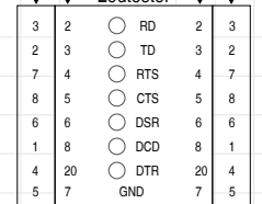
D-Sub 9 with adapters D-Sub 25 direct Ledtester
